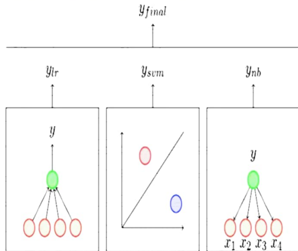
Logistic Regression
